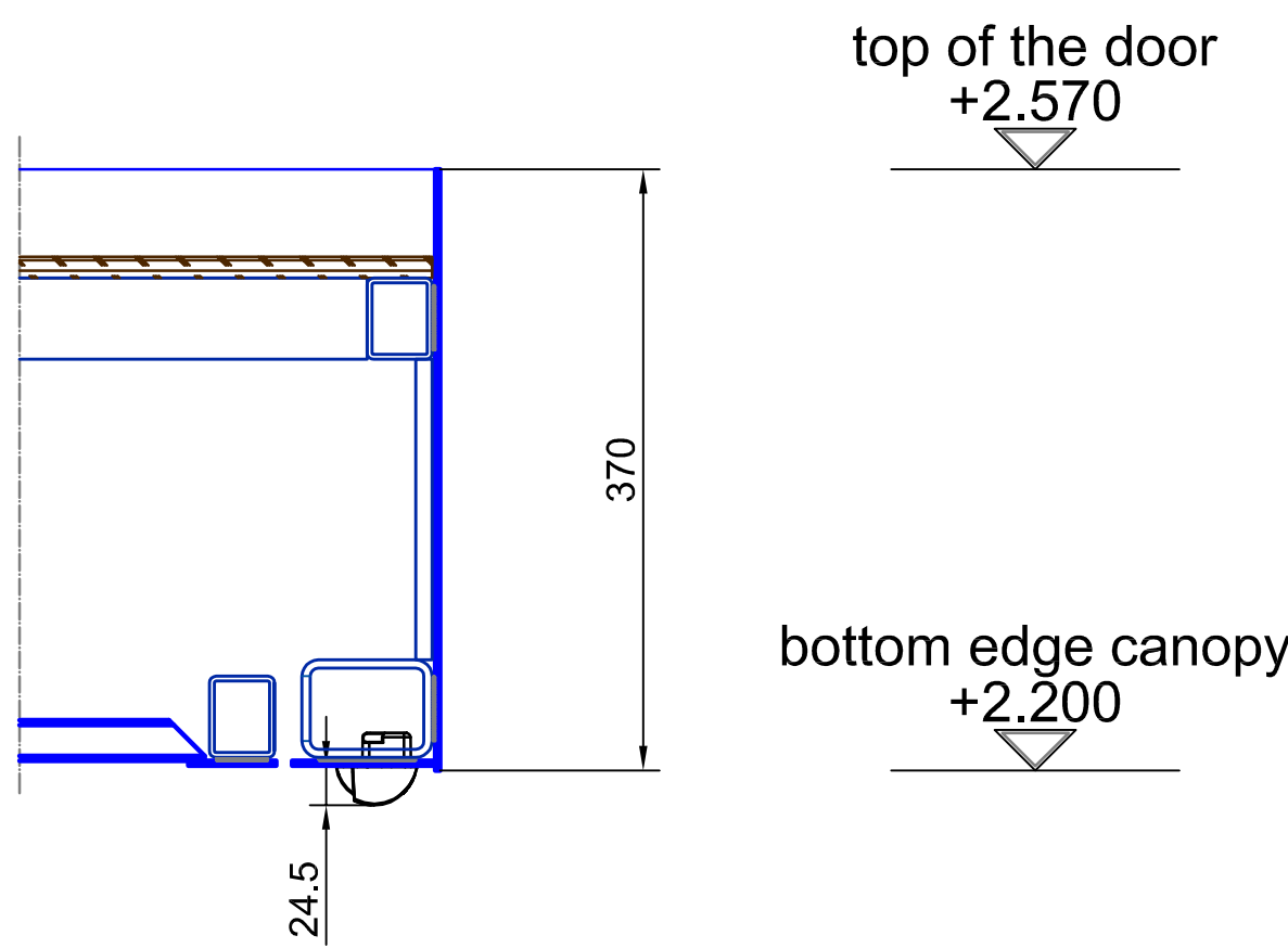
vertical section - passage area / inside
