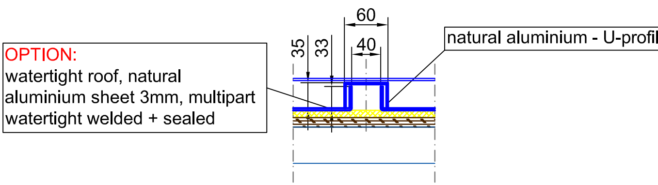
vertical section - watertight roof - multipart
