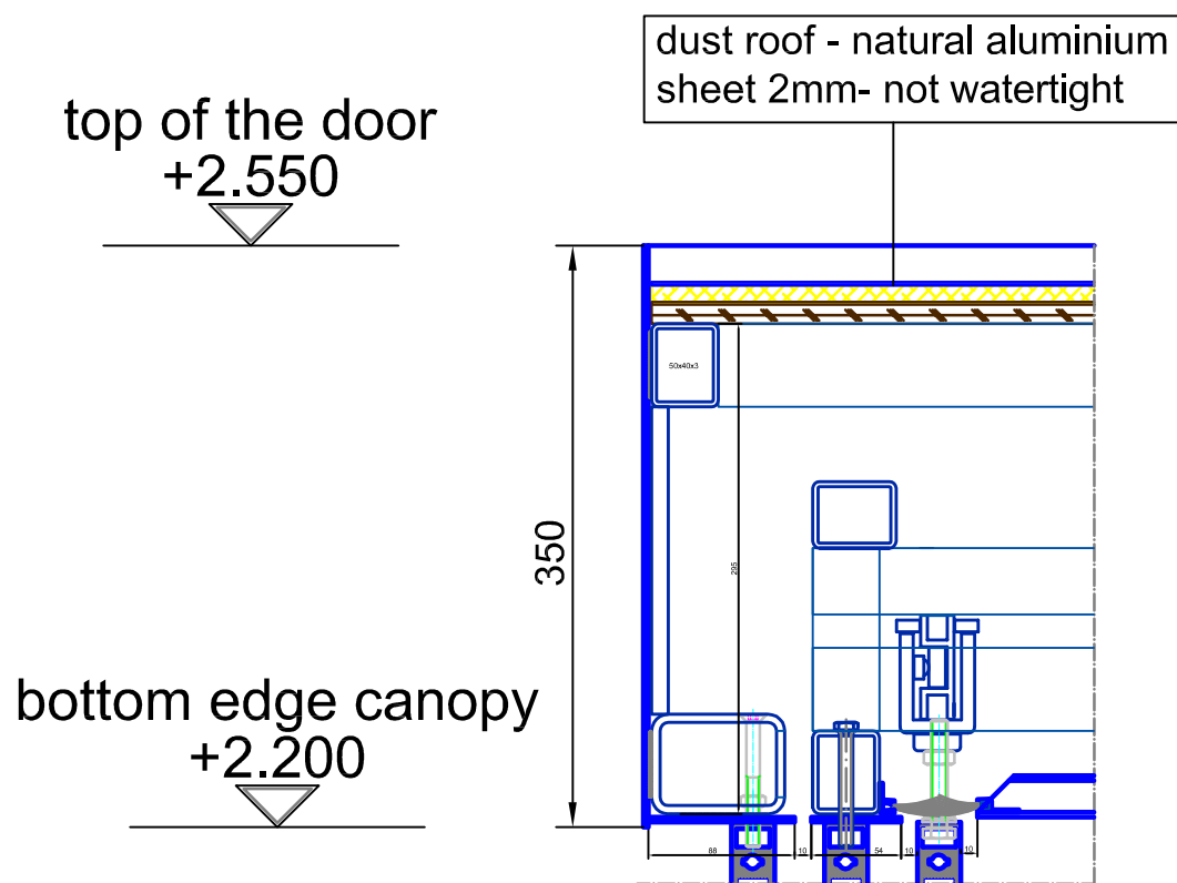
vertical section - dust roof / outside
